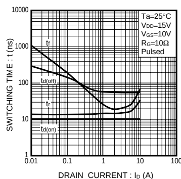
Fig.2 Switching Characteristics
